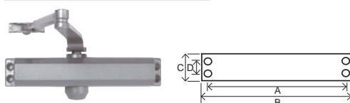
A: 9-1/16" B: 9-5/8" C: 1-13/16" D: 3/4"
